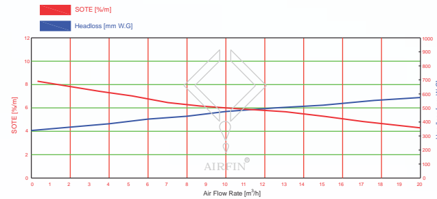
Standard oxygen transfer efficiency (SOTE) and headloss for AIRFIN-3 (92x1020mm) /AIRFIN-2 (80x1020mm performance)
