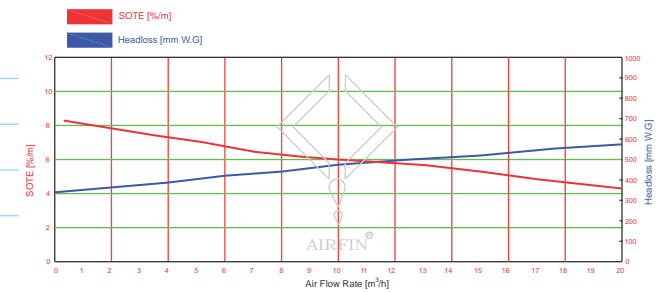
Standard oxygen transfer efficiency (SOTE) and headloss for AIRFIN-3 (92x1020mm) /AIRFIN-2 (80x1020mm performance)
