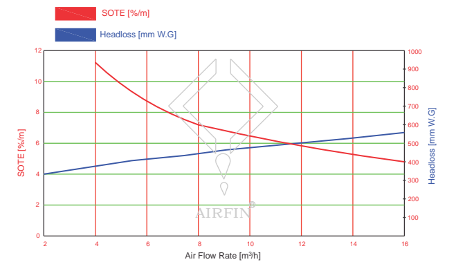
Standard oxygen transfer efficiency (SOTE) and headloss for AIRFIN-1 (65x1020mm) performance
