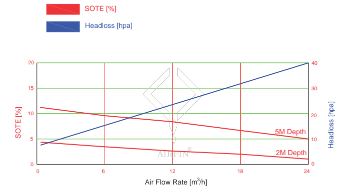
Standard oxygen transfer efficiency (SOTE) and headloss for JCB-80/100/150 performance
