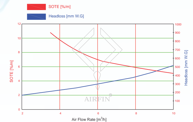
Standard oxygen transfer efficiency (SOTE) and headloss for AIRFIN-600 performance
